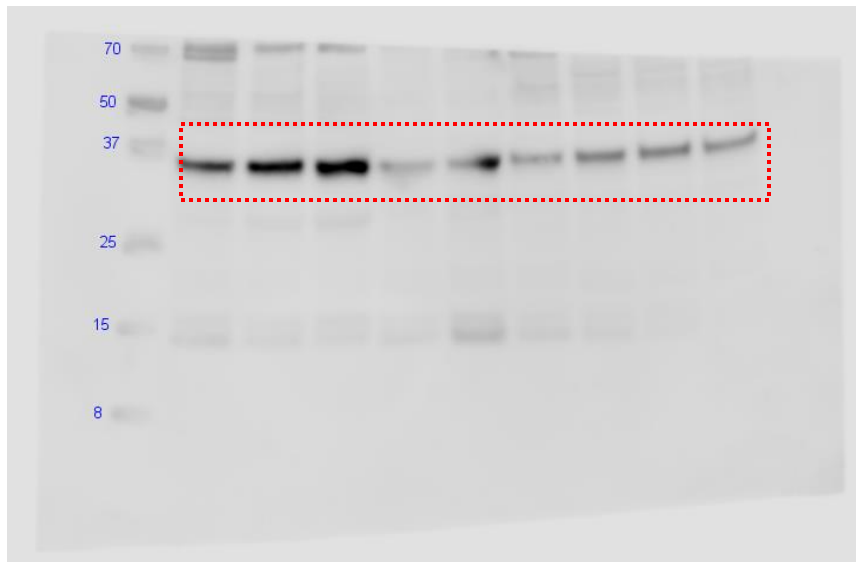
Figure 1D LDHB
