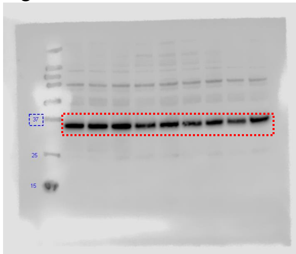
Figure 1D MDH2
