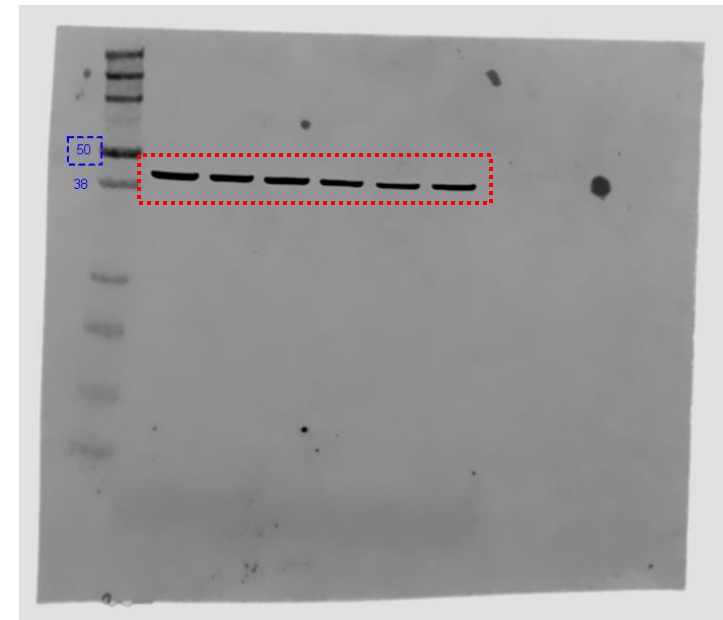
Actin
