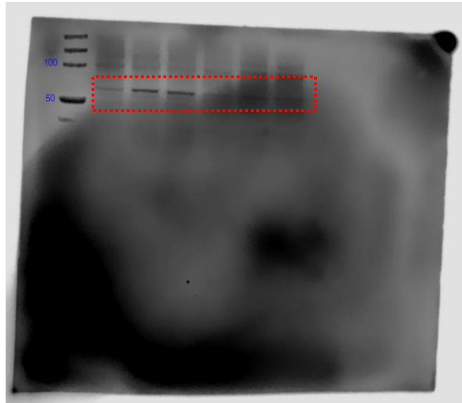
Figure 6A pAMPK
