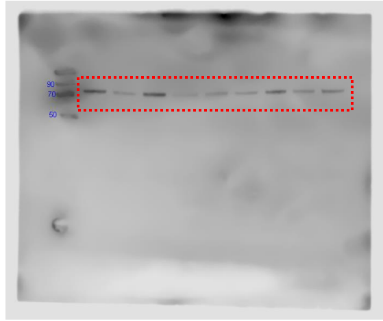
Figure 1D MDH2
