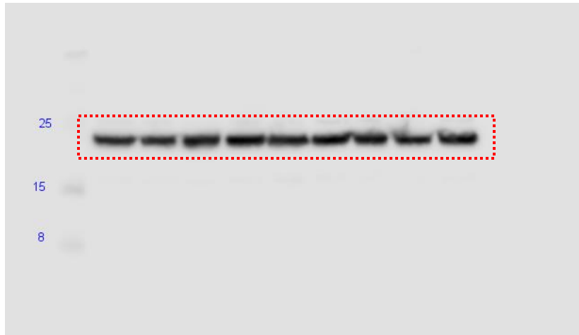
Figure 1D LDHA
