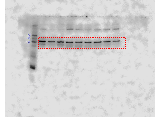
Figure 2J PARKIN
