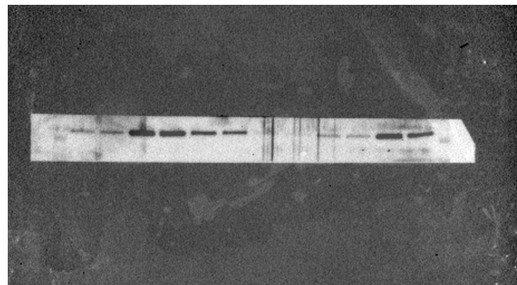
Phospho-JNK (46/54 kDa)
