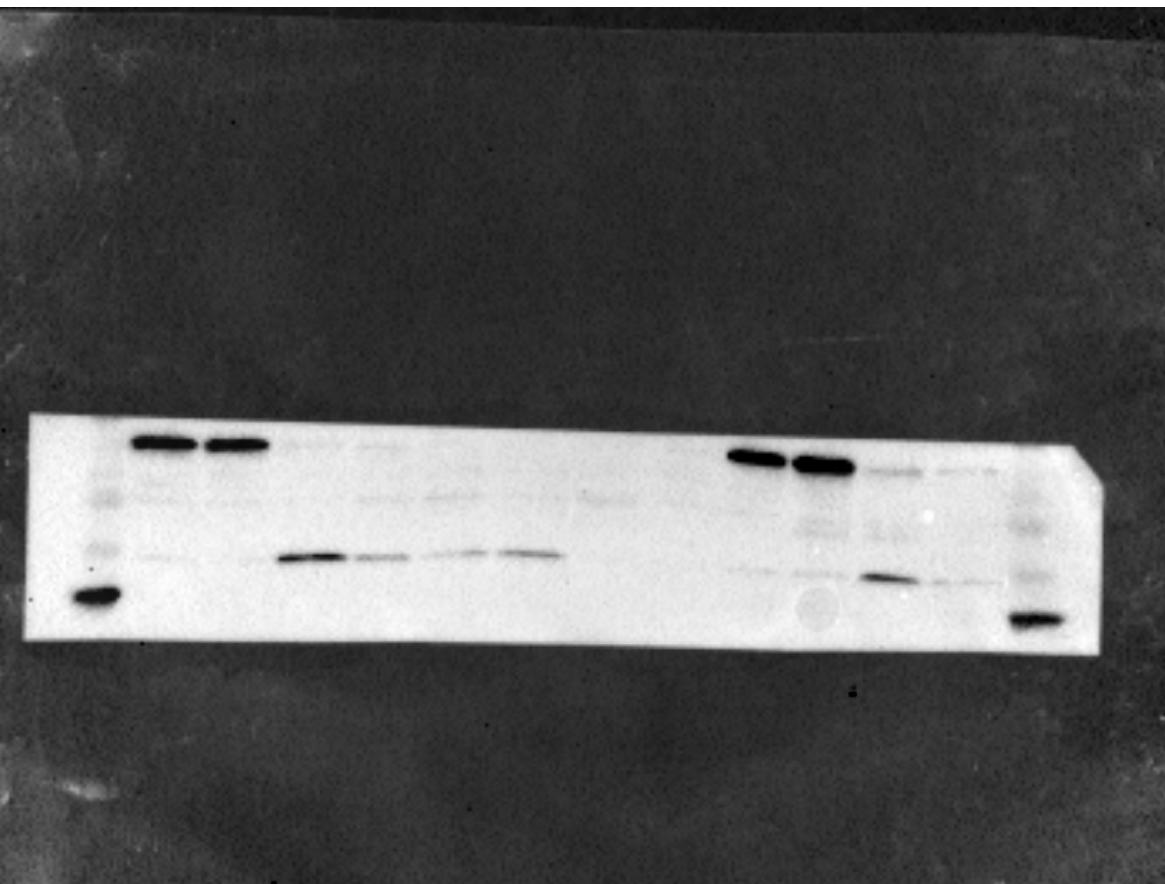
Phospho-S6 (30 kDa)
