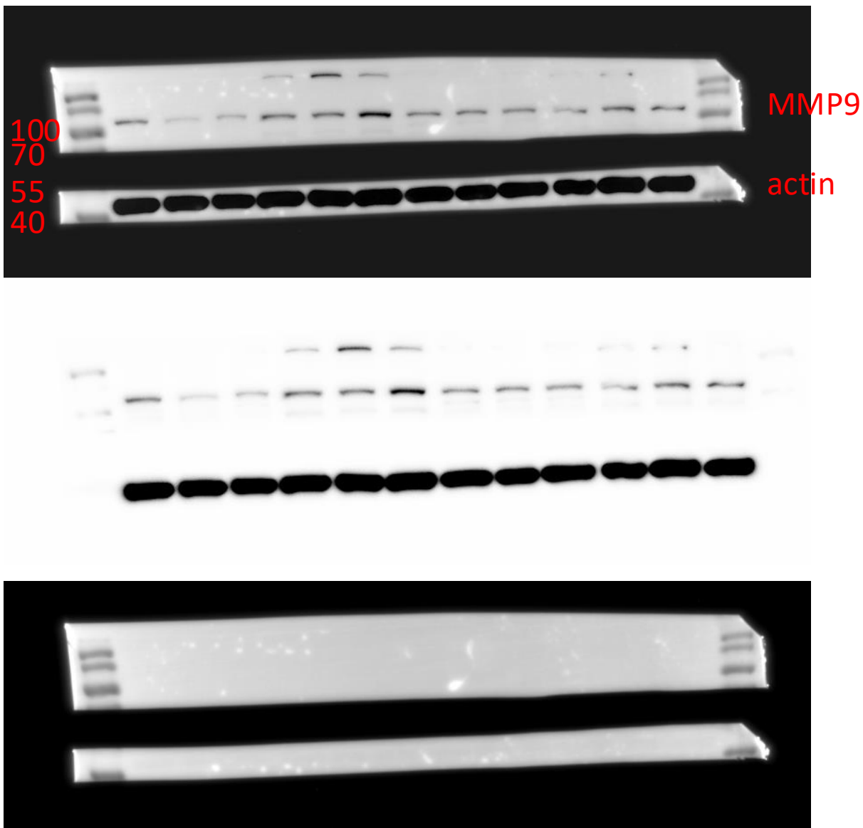
Figure 12 F MMP9
