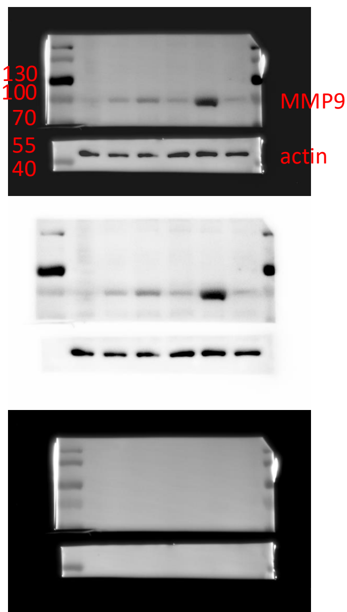
Figure 10 D MMP9
